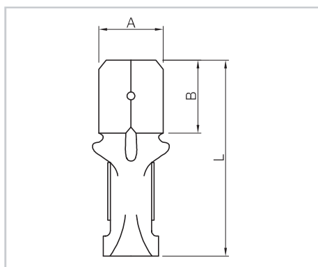
INNESTO MASCHIO MALE CONNECTOR
