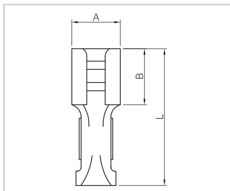
INNESTO FEMMINA FEMALE CONNECTOR
